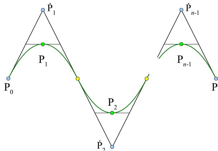
Figure 40: Quadratic spline
