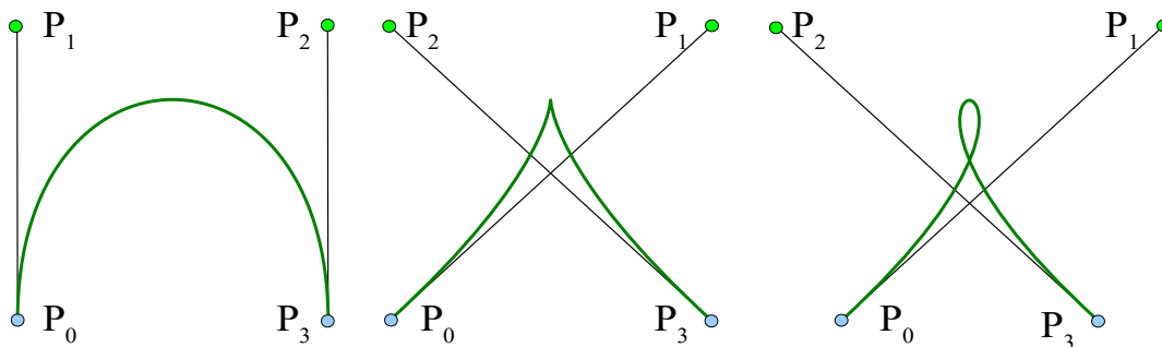
Figure 17: Various cubic Bézier curves
