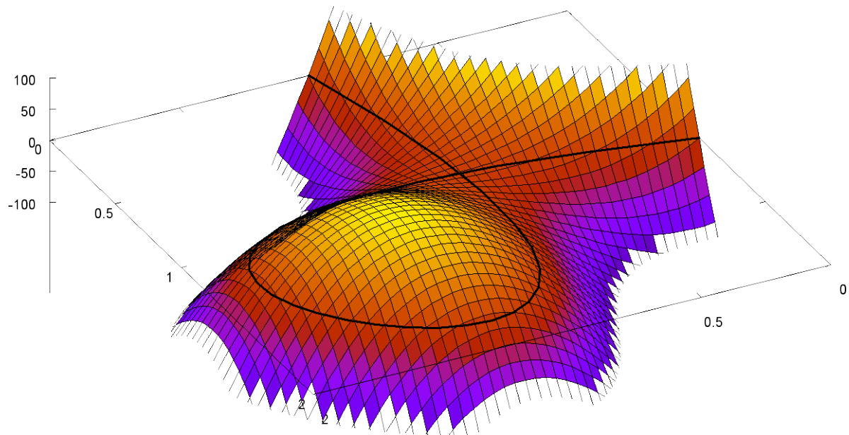
Figure 20: 3D surface plot of a cubic Bézier curve with self-intersection
