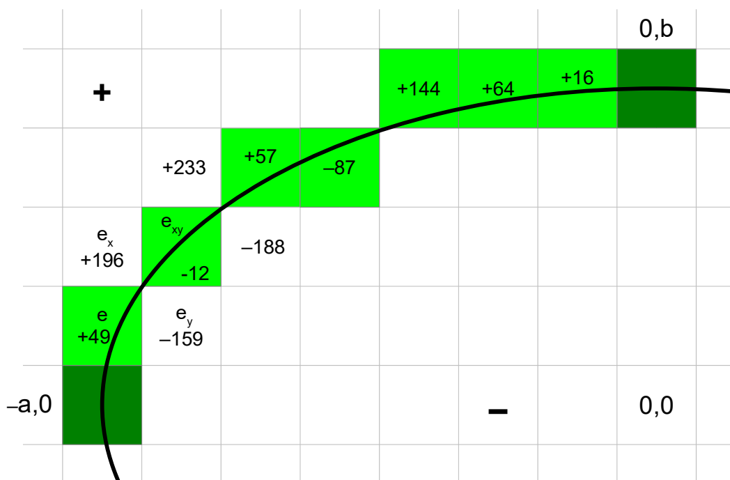
Figure 5: ellipse quadrant with error values for a=7 and b=4
