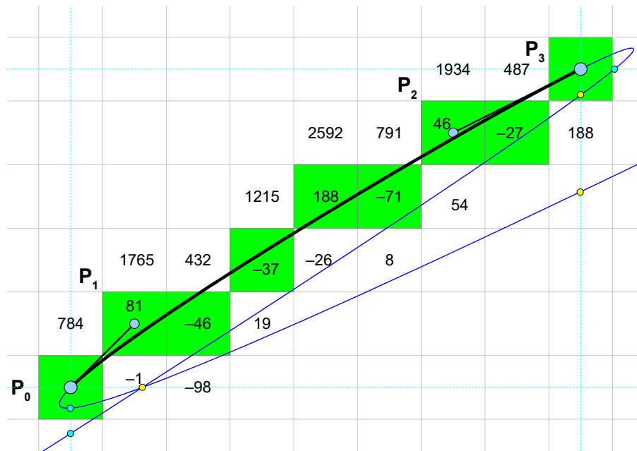
Figure 22: Cubic Bézier with confusing error values
