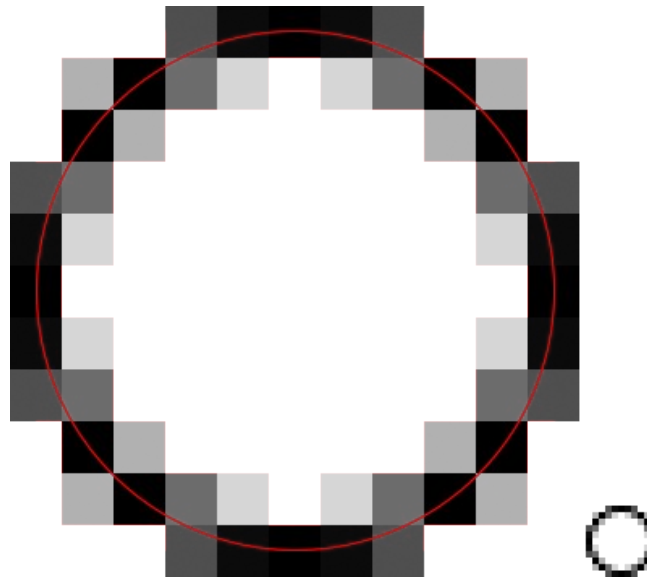
Figure 28: Example of an anti-aliased circle
