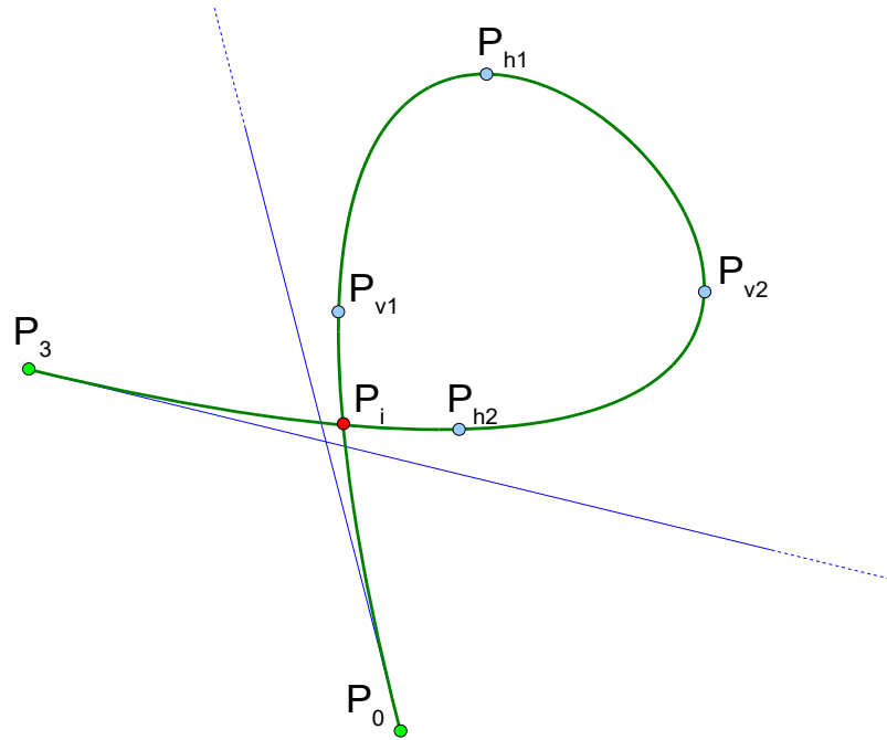
Figure 23: Cubic Bézier curve divided into segments
