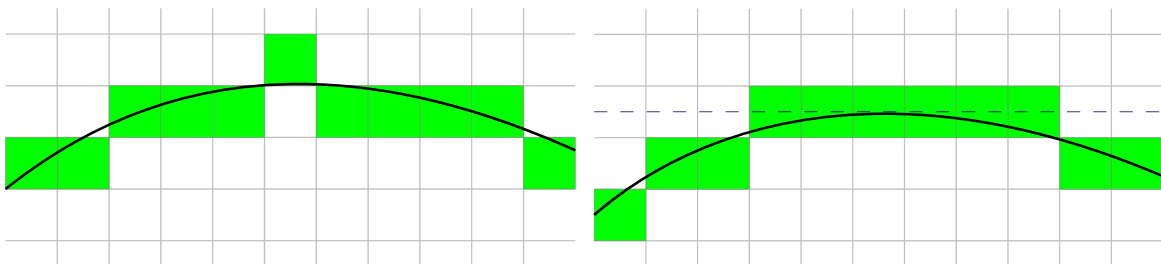
Figure 12: unfavorable curve turn
