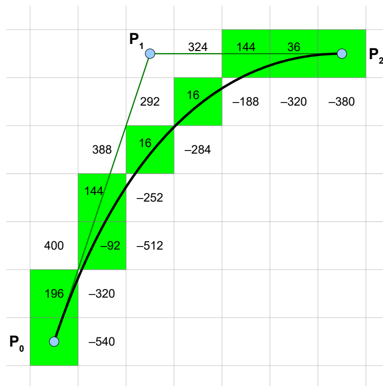
Figure 9: Error values of a quadratic Bézier curve
