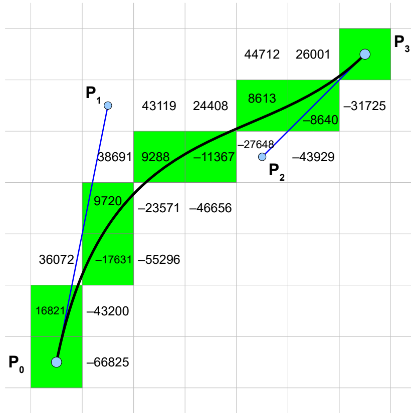
Figure 19: Error values of a cubic Bézier curve
