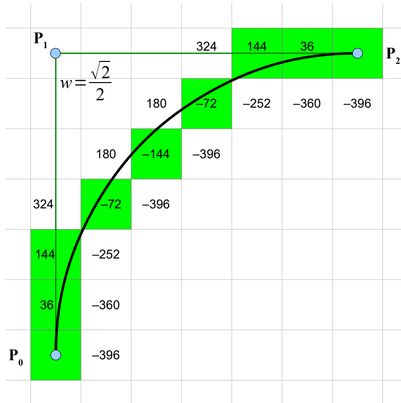
Figure 15: Error values of a quadratic rational Bézier
