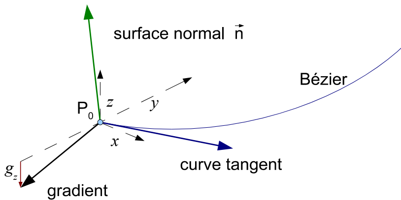
Figure 21: Curve gradient
