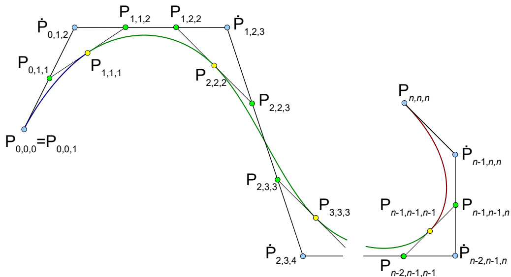
Figure 41: Cubic spline
