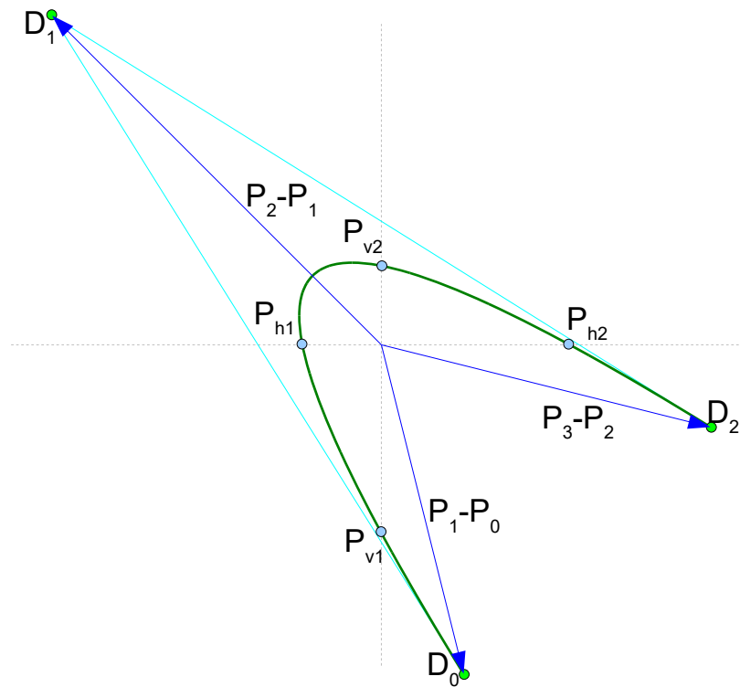
Figure 24: Horizontal and vertical roots of a cubic Bézier
