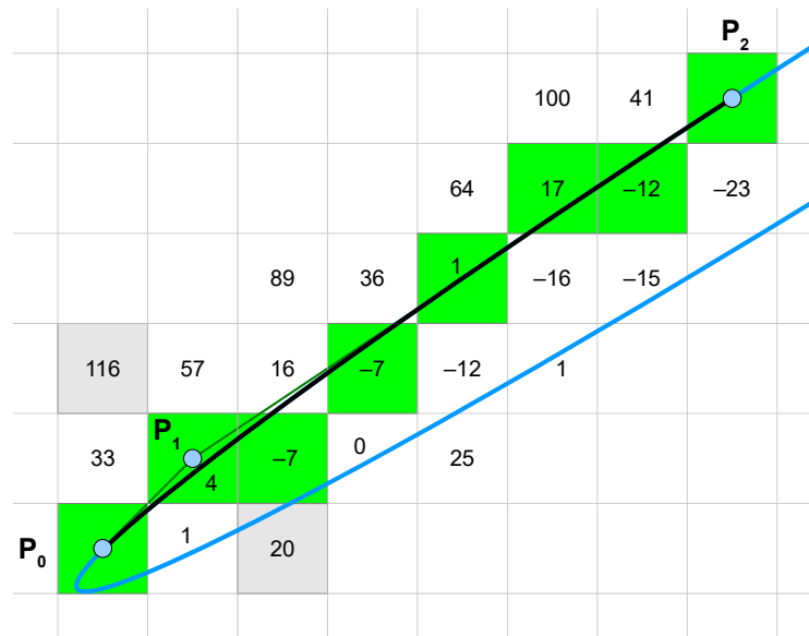
Figure 10: Algorithm in trouble: no path to follow
