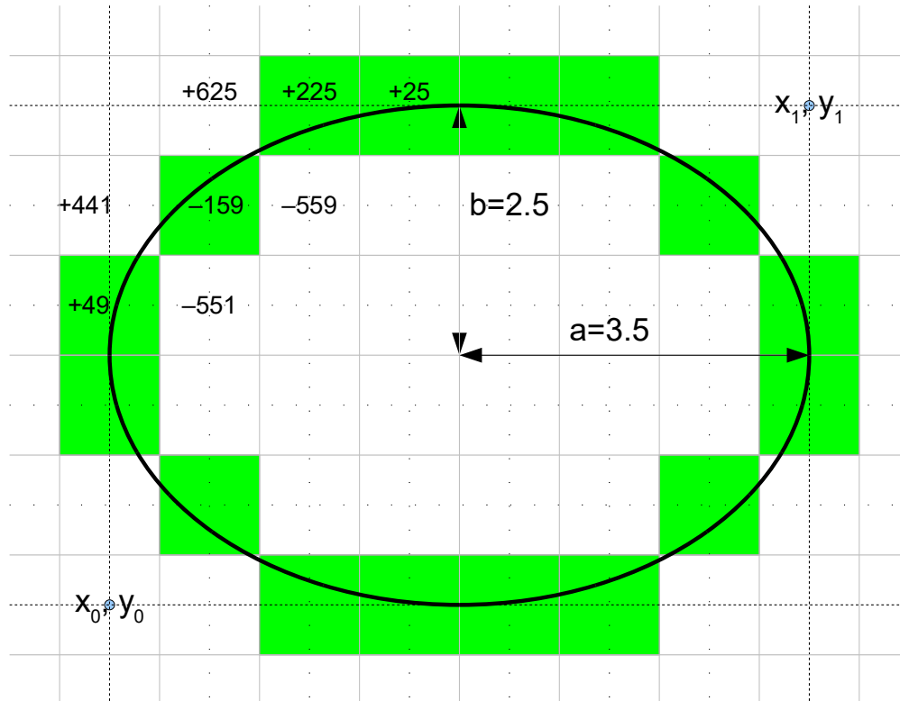
Figure 7: ellipse enclosed by a rectangle of 7x5 pixel
