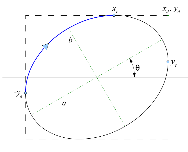
Figure 16: Rotated ellipse
