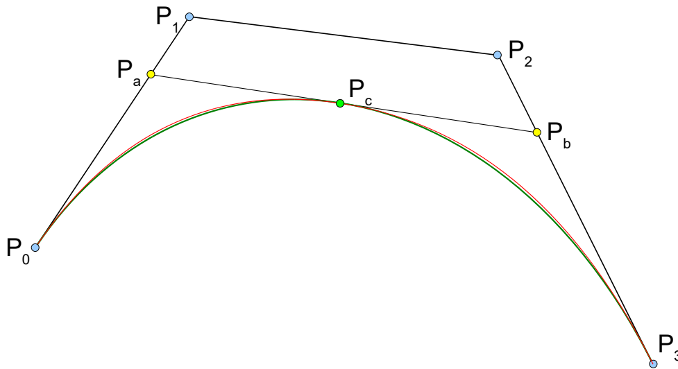
Figure 18: Approximation of a cubic Bézier (red) by two quadratic ones (green)
