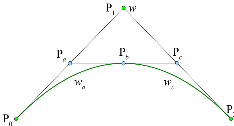
Figure 14: Subdivision of quadratic rational Bézier
