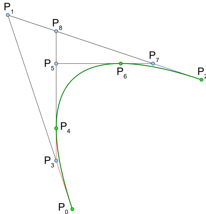
Figure 13: Subdividing a Bézier curve
