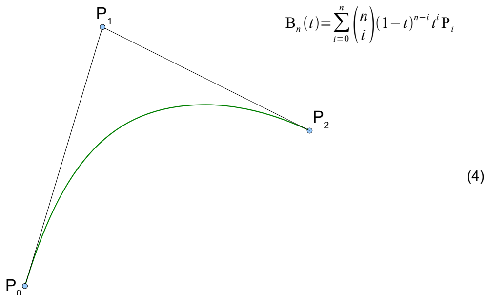
Figure 8: Bézier curve of degree 2
