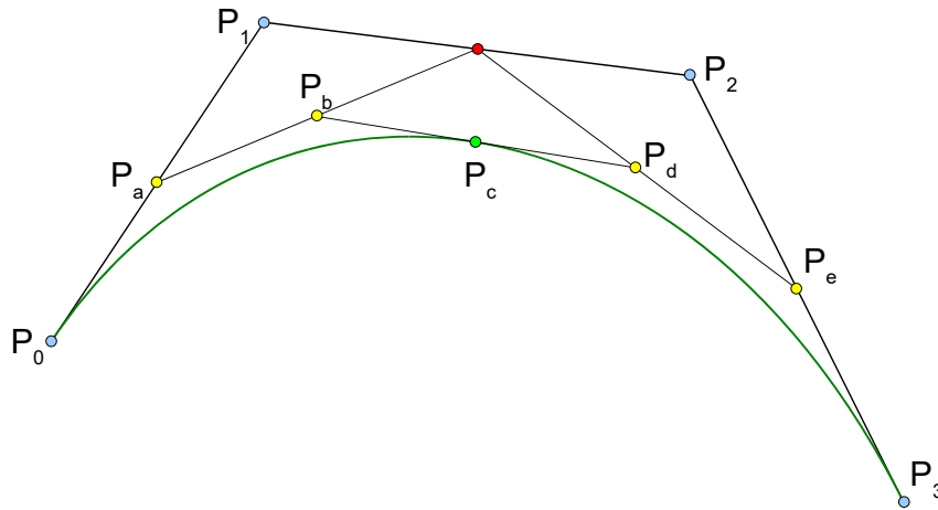
Figure 25: Subdividing a rational cubic Bézier
