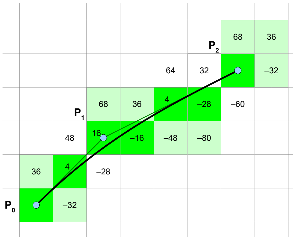
Figure 11: Higher resolution by sub-pixel raster
