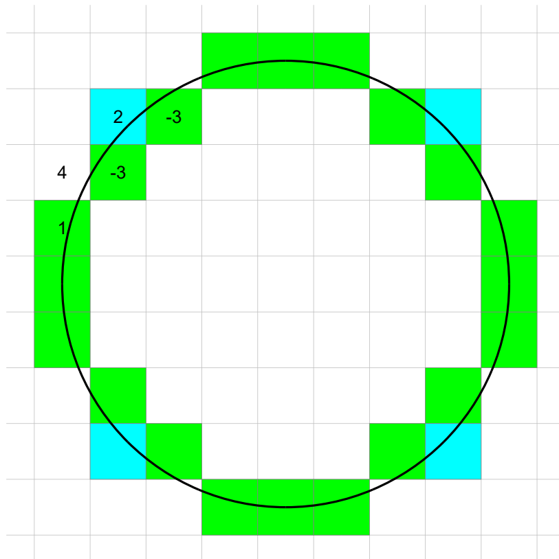
Figure 6: spurious pixel on a circle of radius 4
