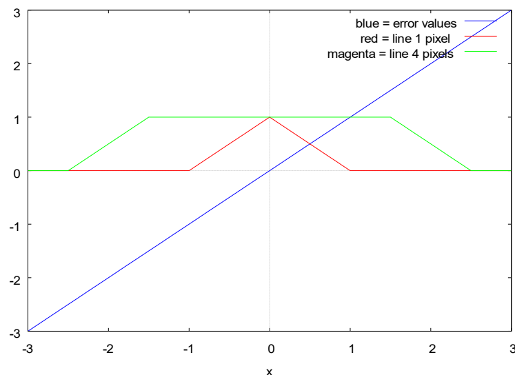
Figure 34: Line thickness according to error values
