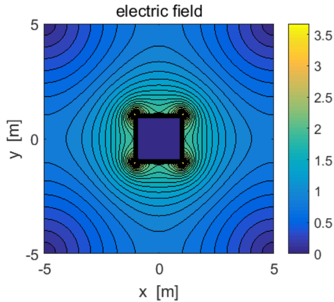
Fig. 5. Contour plot of the magnitude of the electric field. Observe the peaks in the electric field at the corners of the inner square.
